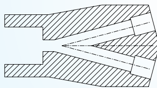
Nozzle
